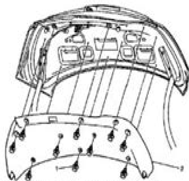
Fig. 45: Rear Compartment Lid Inner Panel Trim & Retainers Courtesy of GENERAL MOTORS COMPANY
