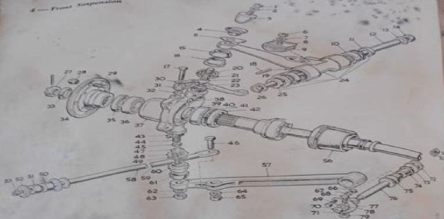
Exploded View of the Front Suspension Components.
