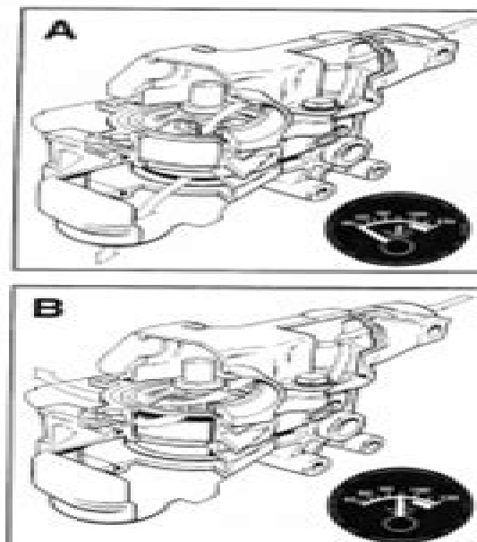
Thermostat
