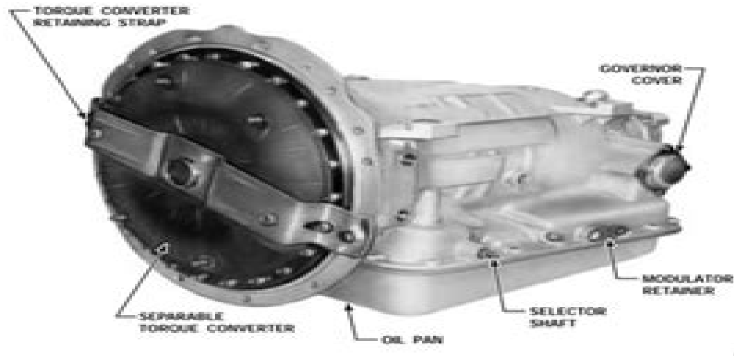
Figure 1-3. AT 543 Automatic Transmission — Left-Front View
