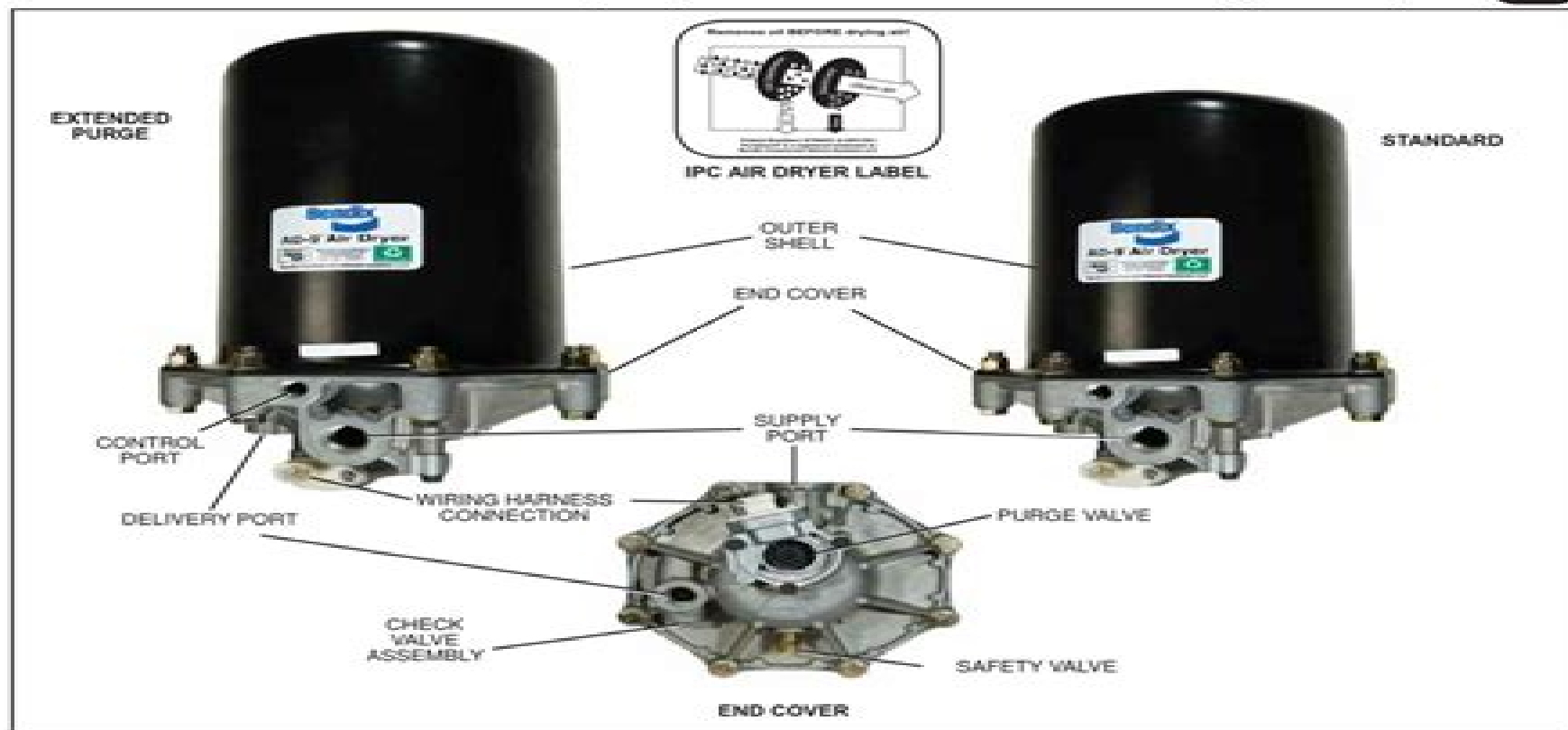
FIGURE 1 - BENDIX® AD-9® AND AD-9® IPC AIR DRYER MODELS
