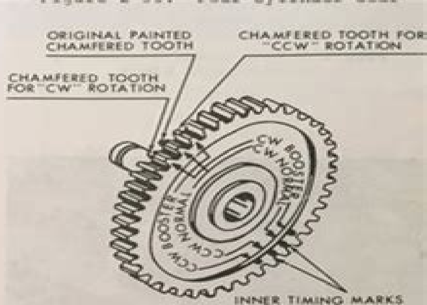
Figure 2-31. Six Cylinder Gear
