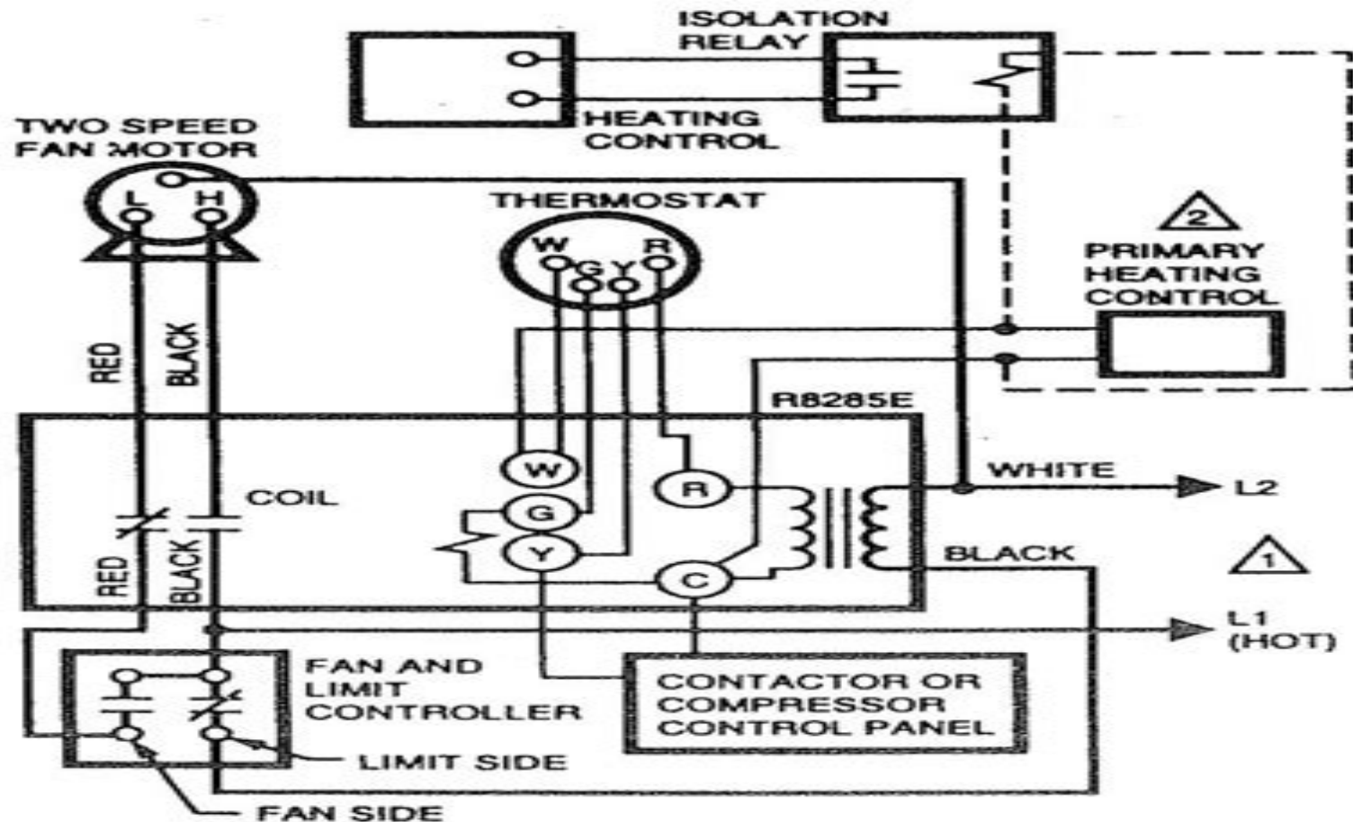
Fig. 6—R8285E typical hookup with two-speed fan and limit controller application.
